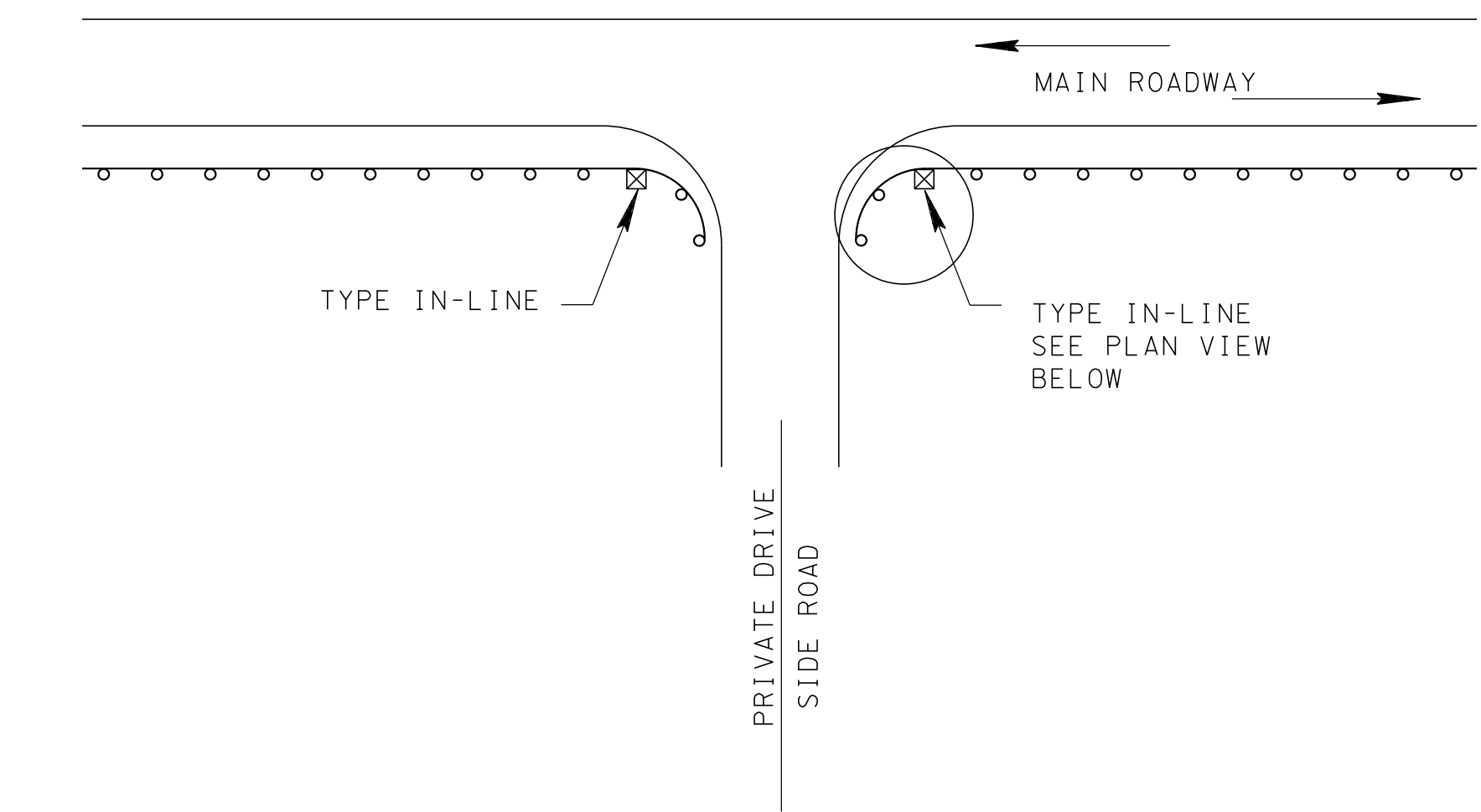
GUARDRAIL TERMINAL ANCHOR (TYPE IN-LINE) APPLICATION
