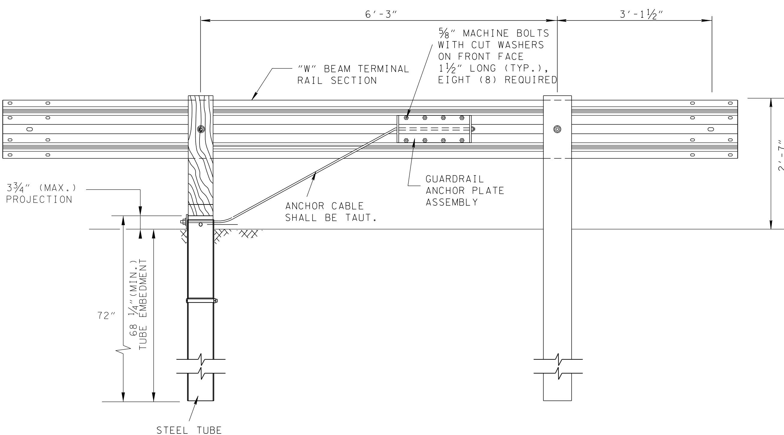
ELEVATION FROM BEHIND GUARDRAIL
